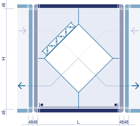
PT Plate heat exchanger Side view – air streams side by side
