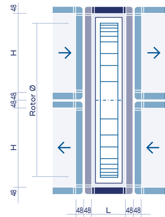
Side view - air streams one above the other
