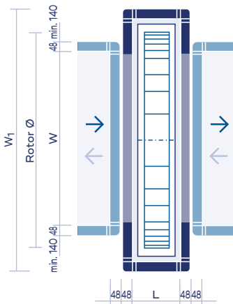
Top view - air streams one above the other / Rotor centred
