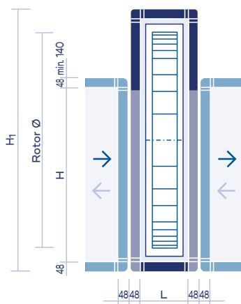
Side view - air streams side by side Rotor 1 side flush
