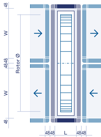
Top view - air streams side by side
