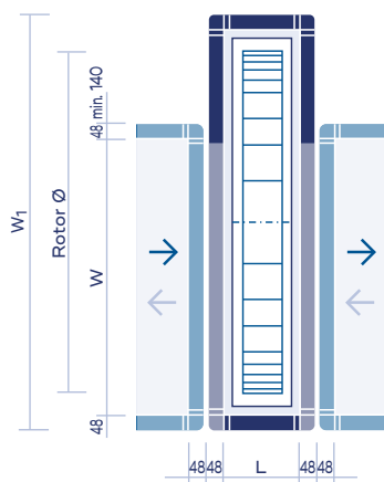
Top view - air streams one above the other / Rotor 1 side flush
