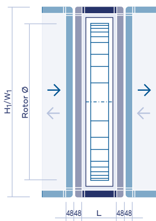
Top view - air streams one above the other Extra wide housing / side view - air streams side by side, with vertical housing extension
