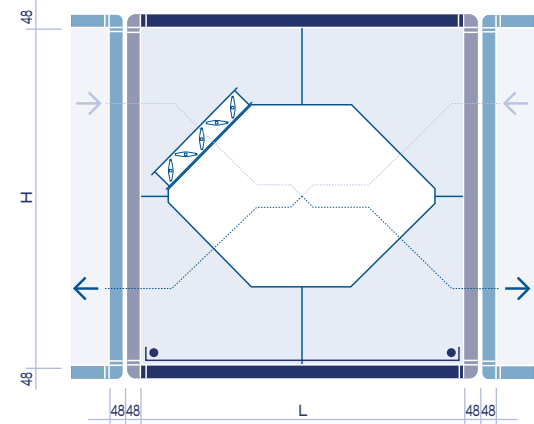
GSWT Counterflow heat exchanger Side view – air streams side by side
