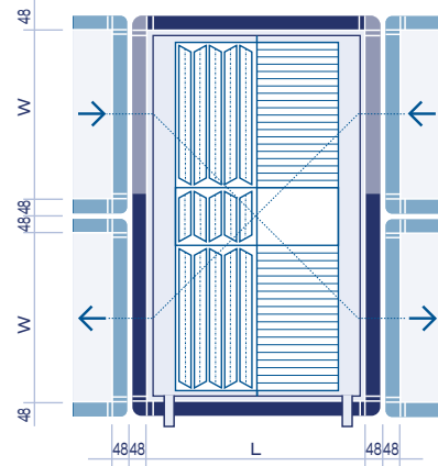
PT plate heat exchanger & GSWT counterflow heat exchanger Top view – air streams side by side
